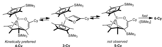
Scheme 2. Reversible C–C reductive elimination and oxidative addition resulting in ejection of [SiMe 3 ] radical.
